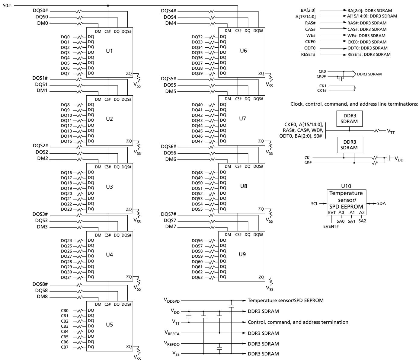
Figure 3: Functional Block Diagram (PCB 1125)
