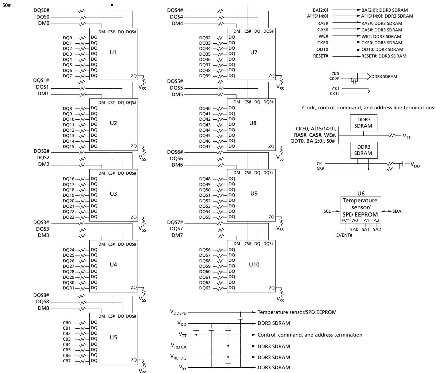
Figure 4: Functional Block Diagram (PCBs1483 & 1568)
