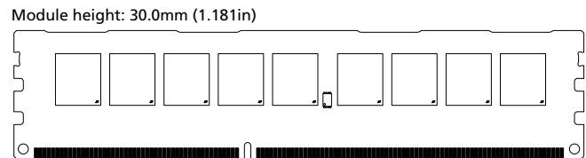
Figure 2: 240-Pin UDIMM (MO-269 R/C D1) PCBs 1483 & 1568
