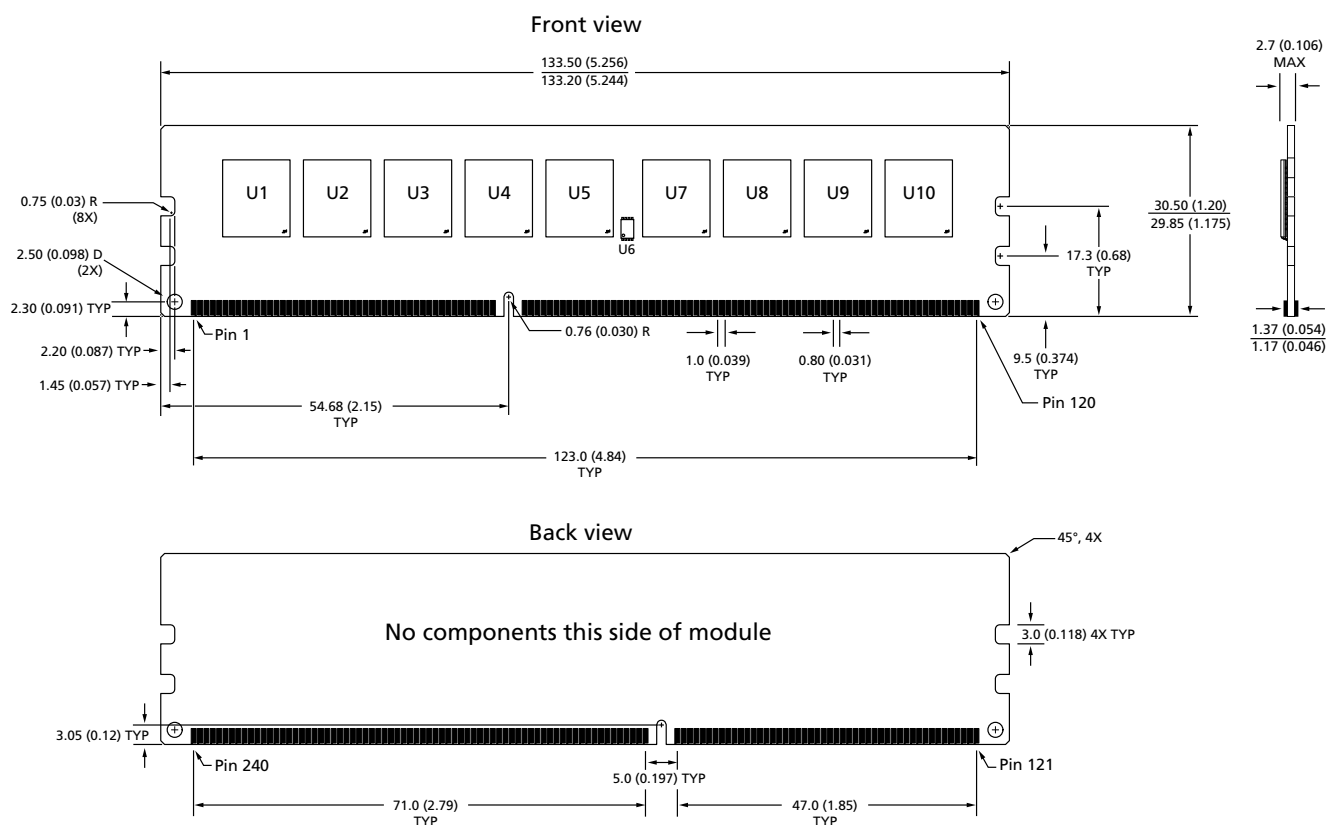
Figure 6: 240-Pin DDR3 UDIMM – PCBs1483 & 1568
