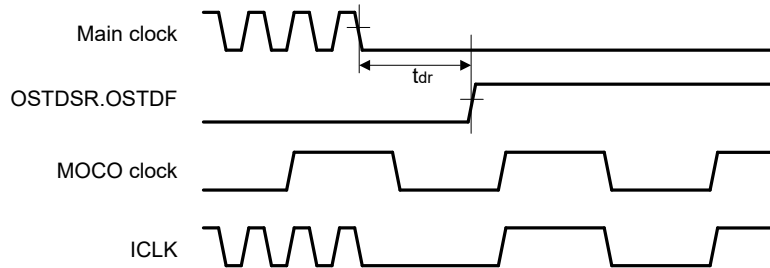
Figure 2.63 Oscillation stop detection timing
