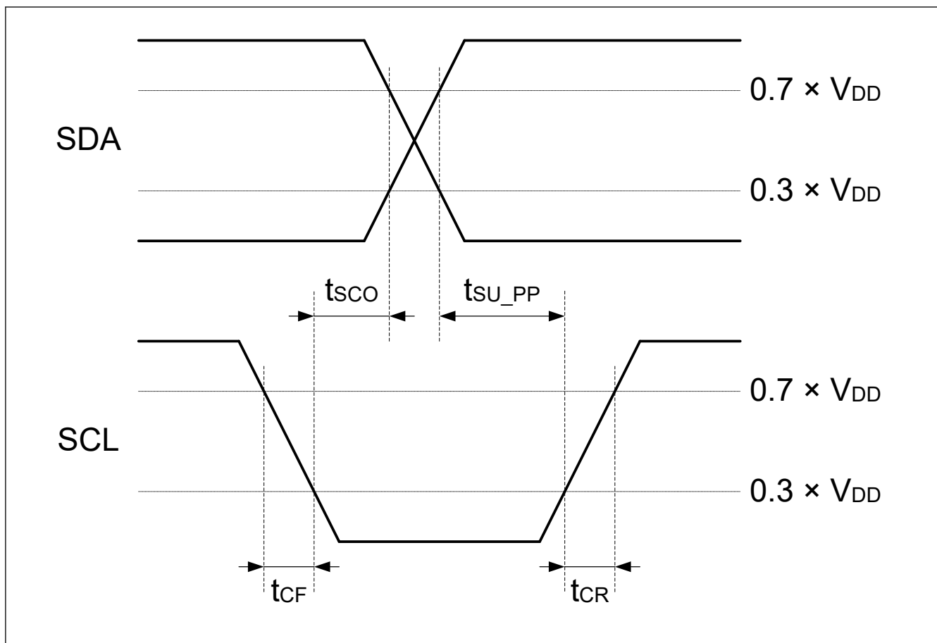
Figure 2.50 I3C slave out timing
