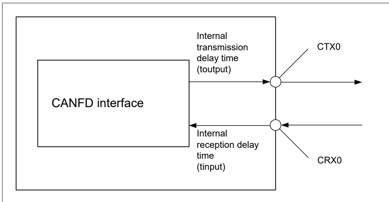
Figure 2.59 CANFD interface condition
