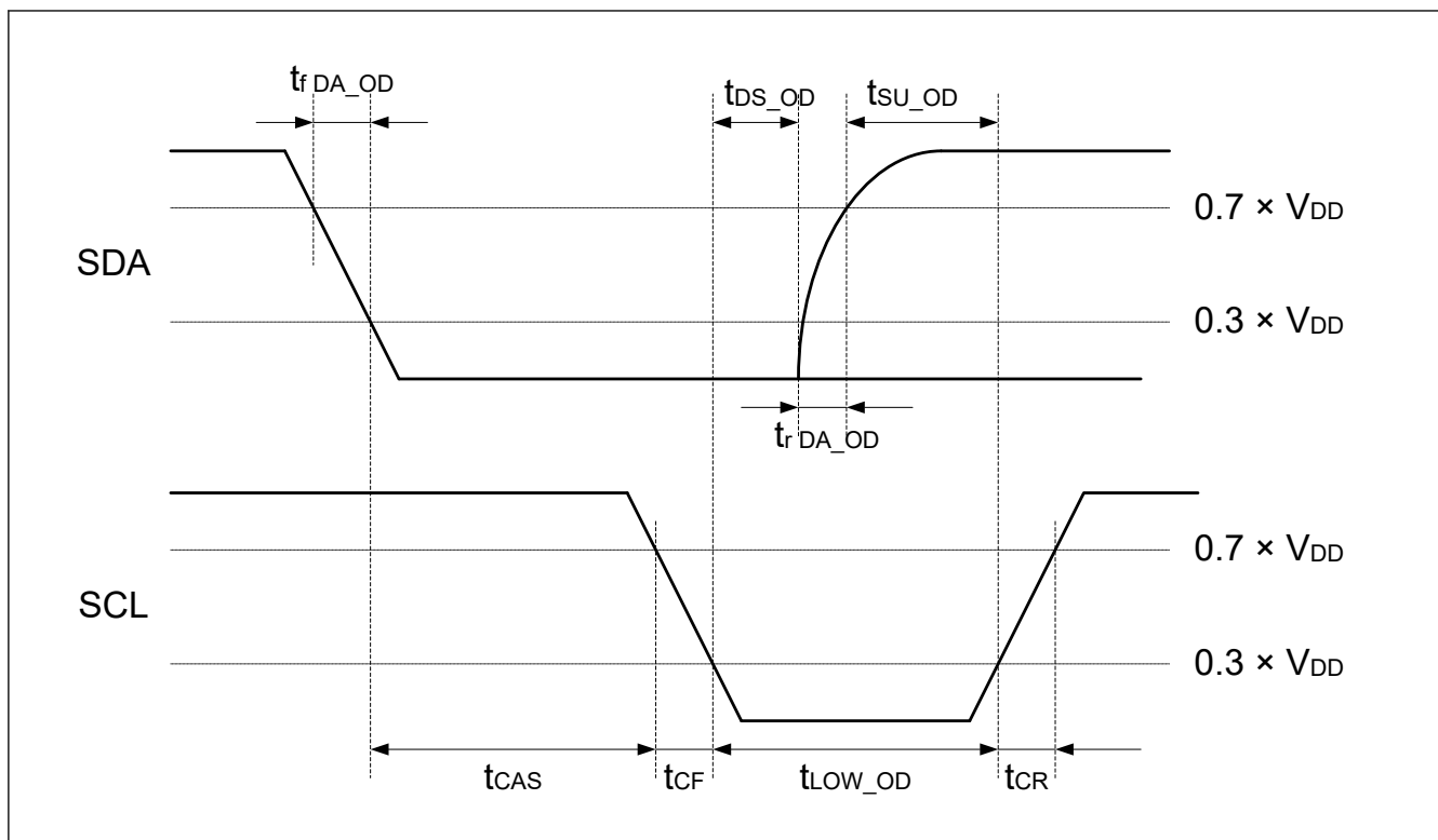
Figure 2.47 I3C START condition timing
