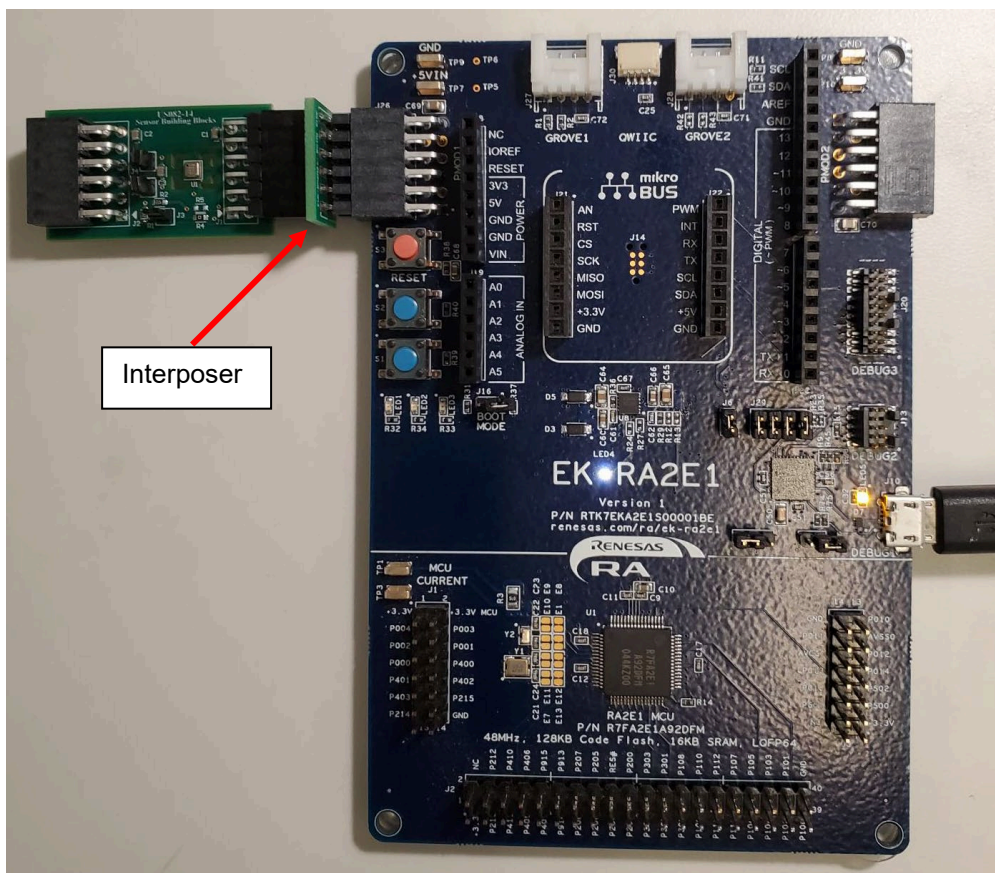
Figure 2. Evaluation Kit Connections using the QCIOT-HS4001POCZ and EK-RA2L1
