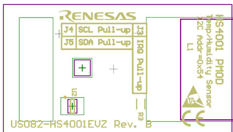
Figure 12. Silkscreen Bottom
