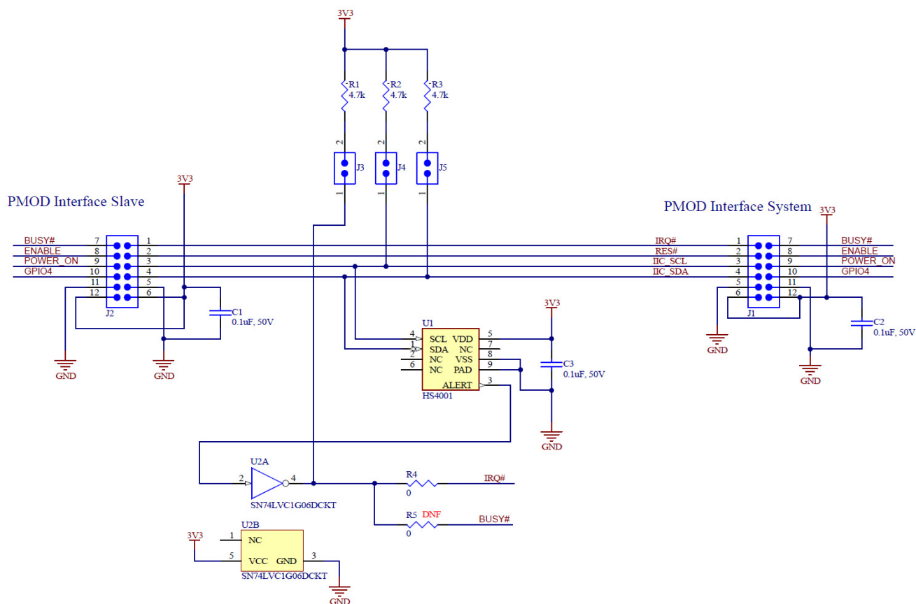
Figure 6. QCIOT-HS4001POCZ Application Schematic
