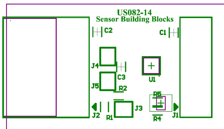
Figure 7. Silkscreen Top
