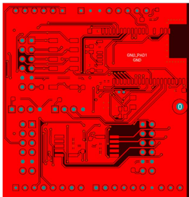
Figure 6. Copper Top
