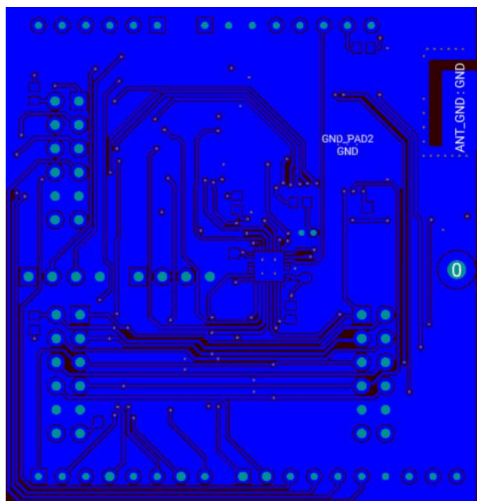
Figure 9. Copper Bottom
