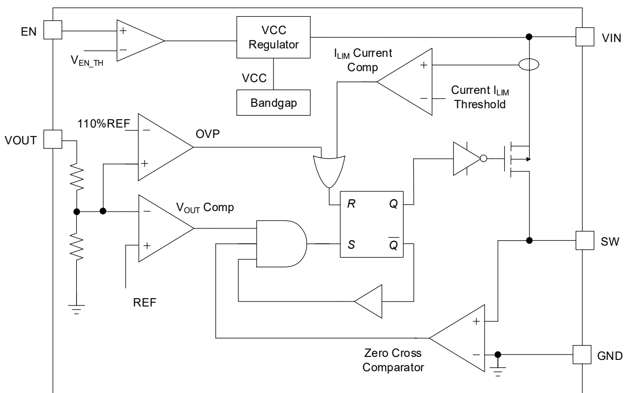
Figure 2. Block Diagram
