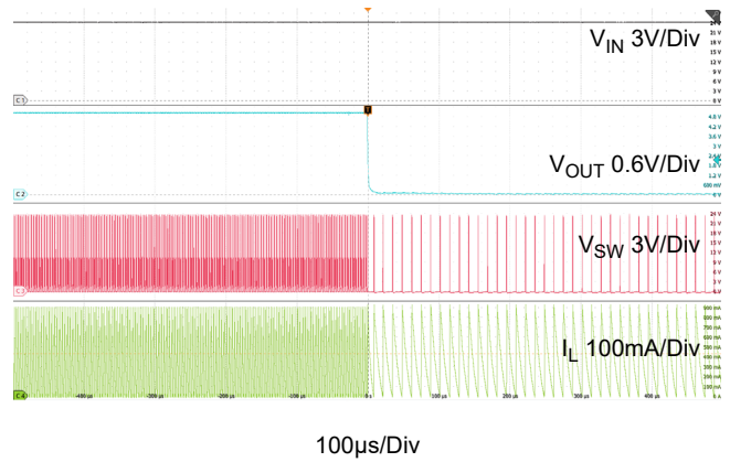
Figure 18. Short-Circuit: RAA211405
