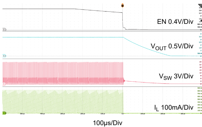
Figure 11. Shutdown through EN: RAA211403
