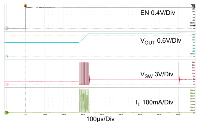
Figure 16. Startup through EN with Pre-Bias (3V) Output Voltage (No Load): RAA211405
