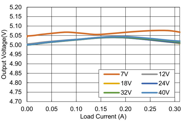
Figure 36. Load Regulation: RAA211405 ( C_{OUT} = 2 \times 22\mu F )
