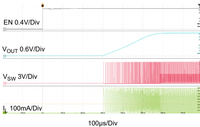
Figure 10. Startup through EN: RAA211405
