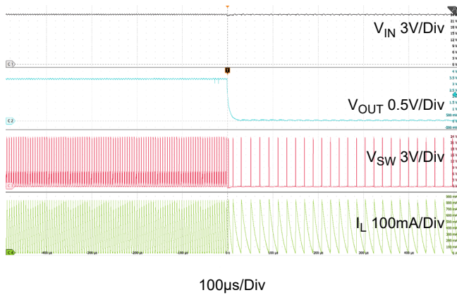
Figure 17. Short-Circuit: RAA211403
