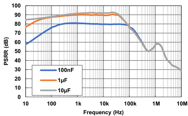
Figure 71. PSRR vs Frequency for Various C_{SET} ( V_{IN} = 5\text{V} , V_{OUT} = 3.3\text{V} , I_{OUT} = 500\text{mA} )
