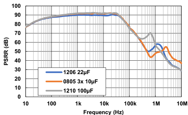
Figure 73. PSRR vs Frequency for Various C_{OUT} ( V_{IN} = 5\text{V} , V_{OUT} = 3.3\text{V} , I_{OUT} = 500\text{mA} )
