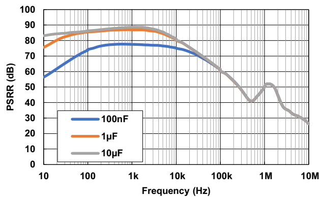
Figure 69. PSRR vs Frequency for Various C_{SET} ( V_{IN} = 4\text{V} , V_{OUT} = 3.3\text{V} , I_{OUT} = 500\text{mA} )
