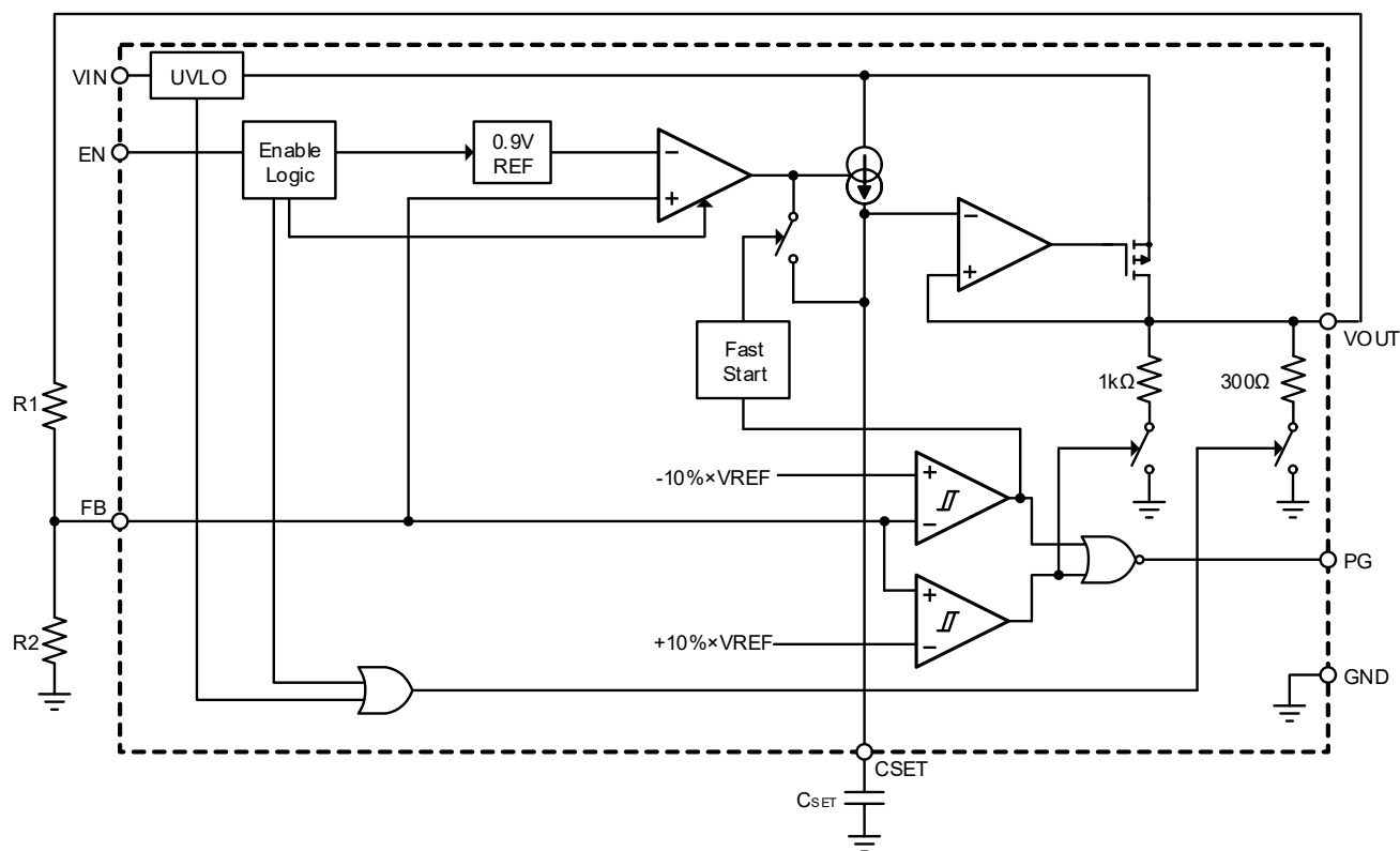
Figure 2. Block Diagram
