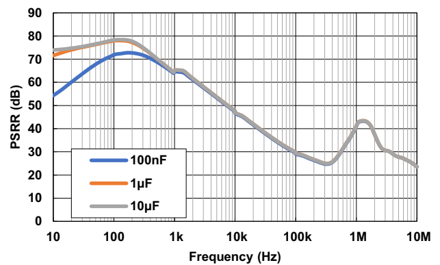
Figure 70. PSRR vs Frequency for Various C_{SET} ( V_{IN} = 4\text{V} , V_{OUT} = 3.3\text{V} , I_{OUT} = 2\text{A} )
