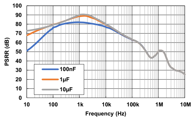
Figure 72. PSRR vs Frequency for Various C_{SET} ( V_{IN} = 5\text{V} , V_{OUT} = 3.3\text{V} , I_{OUT} = 2\text{A} )
