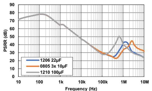
Figure 74. PSRR vs Frequency for Various C_{OUT} ( V_{IN} = 4\text{V} , V_{OUT} = 3.3\text{V} , I_{OUT} = 2\text{A} )
