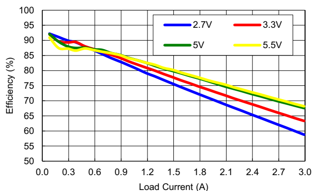
Figure 6. Efficiency vs Load, V_{OUT} = 0.6V
