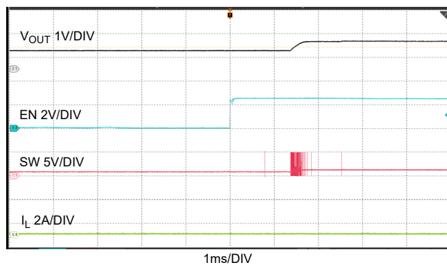
Figure 25. Pre-Bias On, No Load
