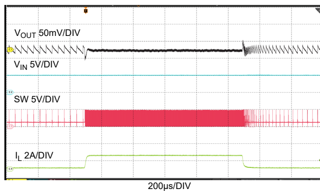
Figure 23. Load Transition, 0A->1.5A
