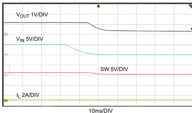
Figure 15. Shutdown at 0A
