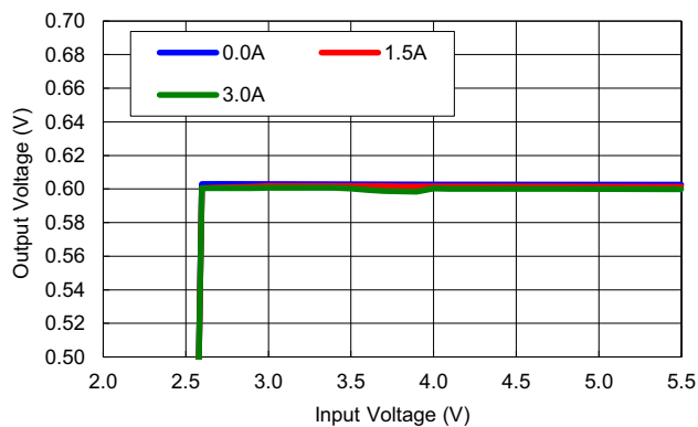
Figure 12. Line Regulation, V_{\text{OUT}} = 0.6\text{V}
