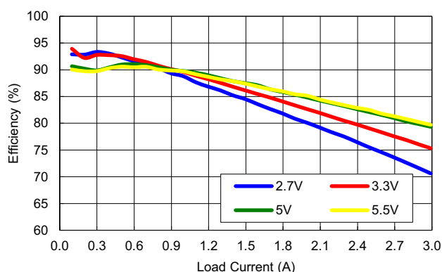
Figure 5. Efficiency vs Load, V_{OUT} = 1.2V
