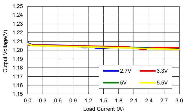
Figure 8. V_{OUT} Regulation vs Load, V_{OUT} = 1.2V
