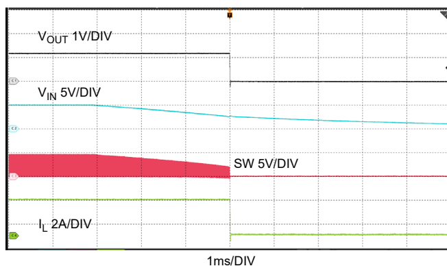
Figure 17. Shutdown at 3A
