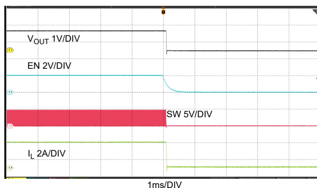
Figure 21. EN Off at 3A
