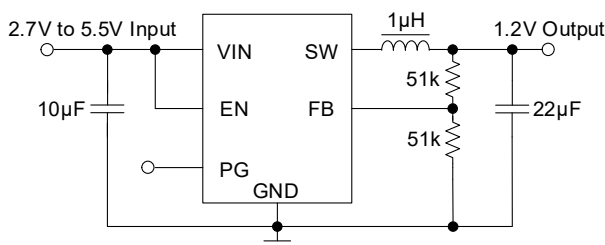
Figure 1. Typical Application
