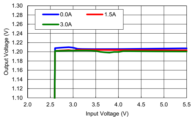
Figure 11. Line Regulation, V_{\text{OUT}} = 1.2\text{V}
