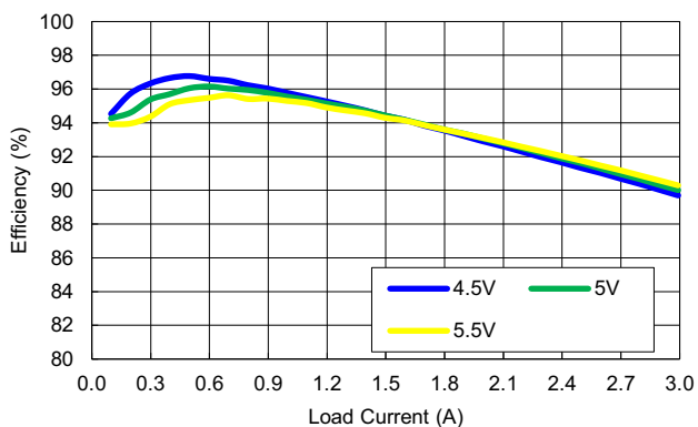
Figure 7. Efficiency vs Load, V_{OUT} = 3.3V
