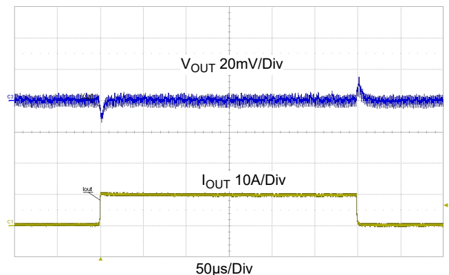
Figure 28. Transient Response, V_{IN} = 12V , V_{OUT} = 1.2V , 0A to 15A, 5A/μs Step Load, C_{OUT} = 7 \times 47\mu F Ceramic + 2 \times 470\mu F Polymer Capacitor
