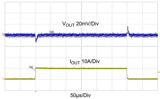
Figure 26. Transient Response, C_{IN} = 12V , V_{OUT} = 0.8V , 0A to 15A to 0A, 5A/μs Step Load, C_{OUT} = 10 \times 47\mu F Ceramic + 2 \times 470\mu F Polymer Capacitor
