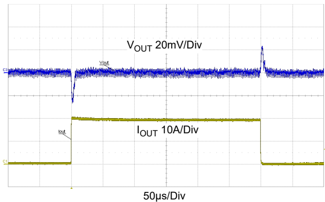
Figure 27. Transient Response, V_{IN} = 12V , V_{OUT} = 0.8V , 0A to 30A to 0A, 5A/μs Step Load, C_{OUT} = 10 \times 47\mu F Ceramic + 2 \times 470\mu F Polymer Capacitor
