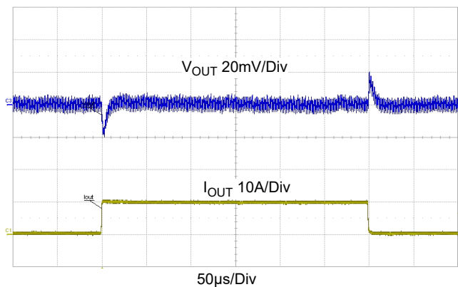
Figure 29. Transient Response, V_{IN} = 12V , V_{OUT} = 1.8V , 0A to 10A to 0A, 5A/μs Step Load, C_{OUT} = 7 \times 47\mu F Ceramic + 2 \times 470\mu F Polymer Capacitor
