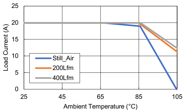
Figure 34. Thermal Derating Curve, V_{IN} = 12V , V_{OUT} = 1.2V , f_{SW} = 550kHz .
