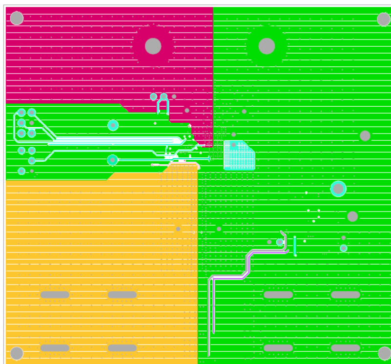
Figure 12. Inner Layer 3
