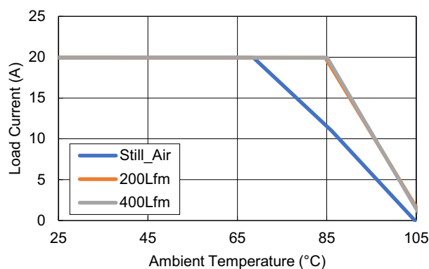
Figure 36. Thermal Derating Curve, V_{IN} = 12V , V_{OUT} = 3.3V , f_{SW} = 700kHz
