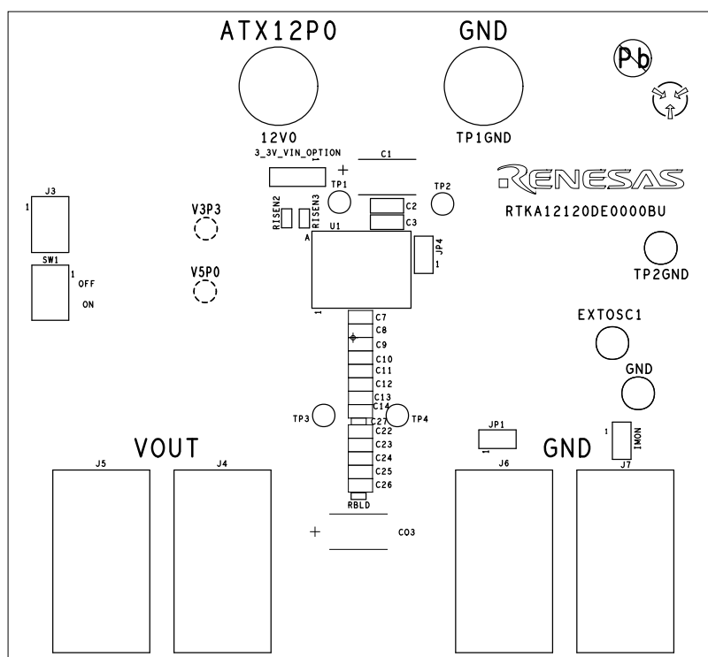
Figure 9. Silkscreen Top
