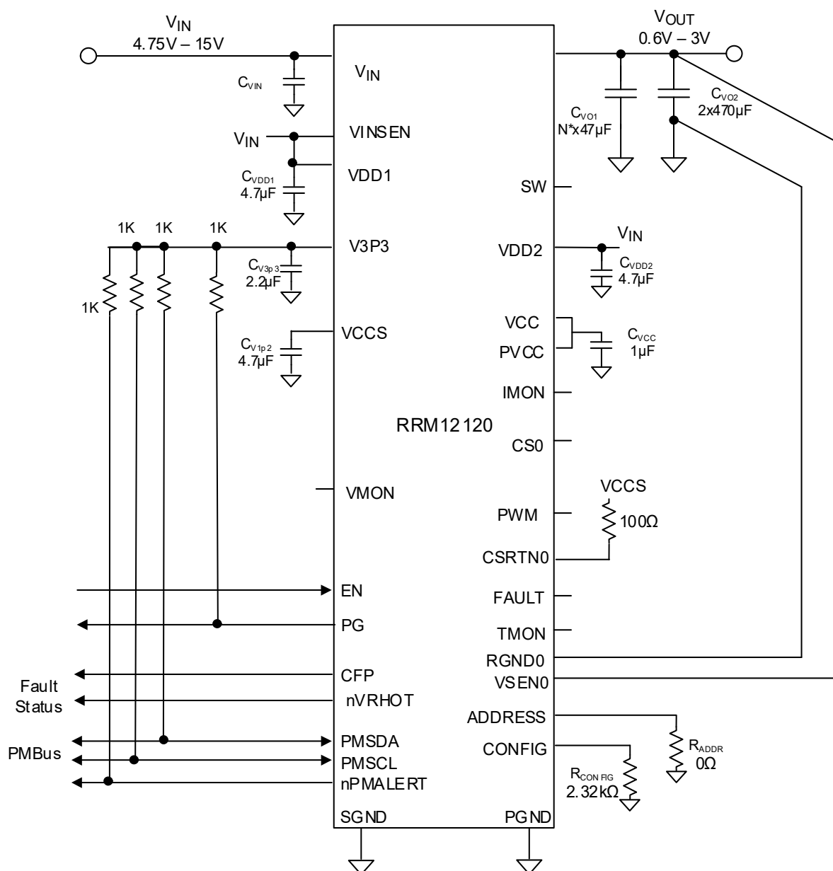
Figure 1. Block Diagram
