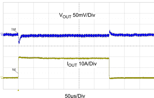
Figure 30. Transient Response, V_{IN} = 12V , V_{OUT} = 3.3V , 0A to 20A to 0A, 5A/μs Step Load, C_{OUT} = 15 \times 47\mu F Ceramic + 2 \times 470\mu F Polymer Capacitor
