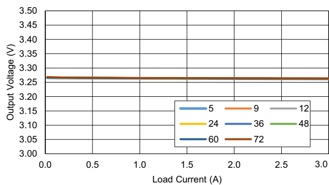
Figure 11. Load Regulation
