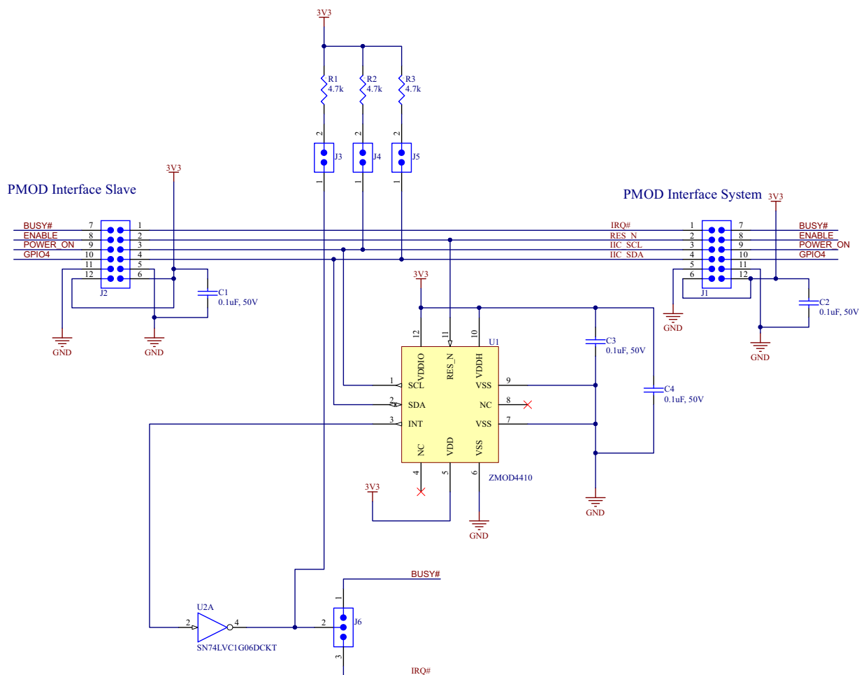
Figure 7. US082-ZMOD4410EVZ Schematic
