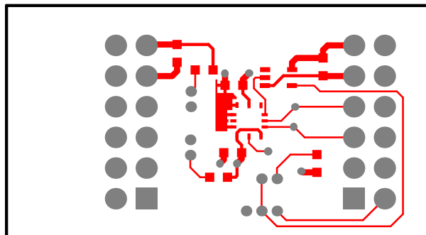
Figure 9. Top Layer
