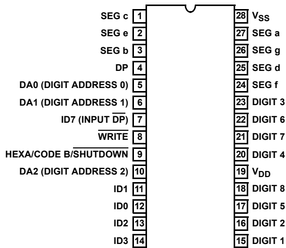
ICM7228C (PDIP, SOIC) COMMON ANODE TOP VIEW
