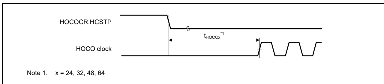
Figure 2.29 HOCO clock oscillator start timing (started by setting HOCOCCR.HCSTP bit)
