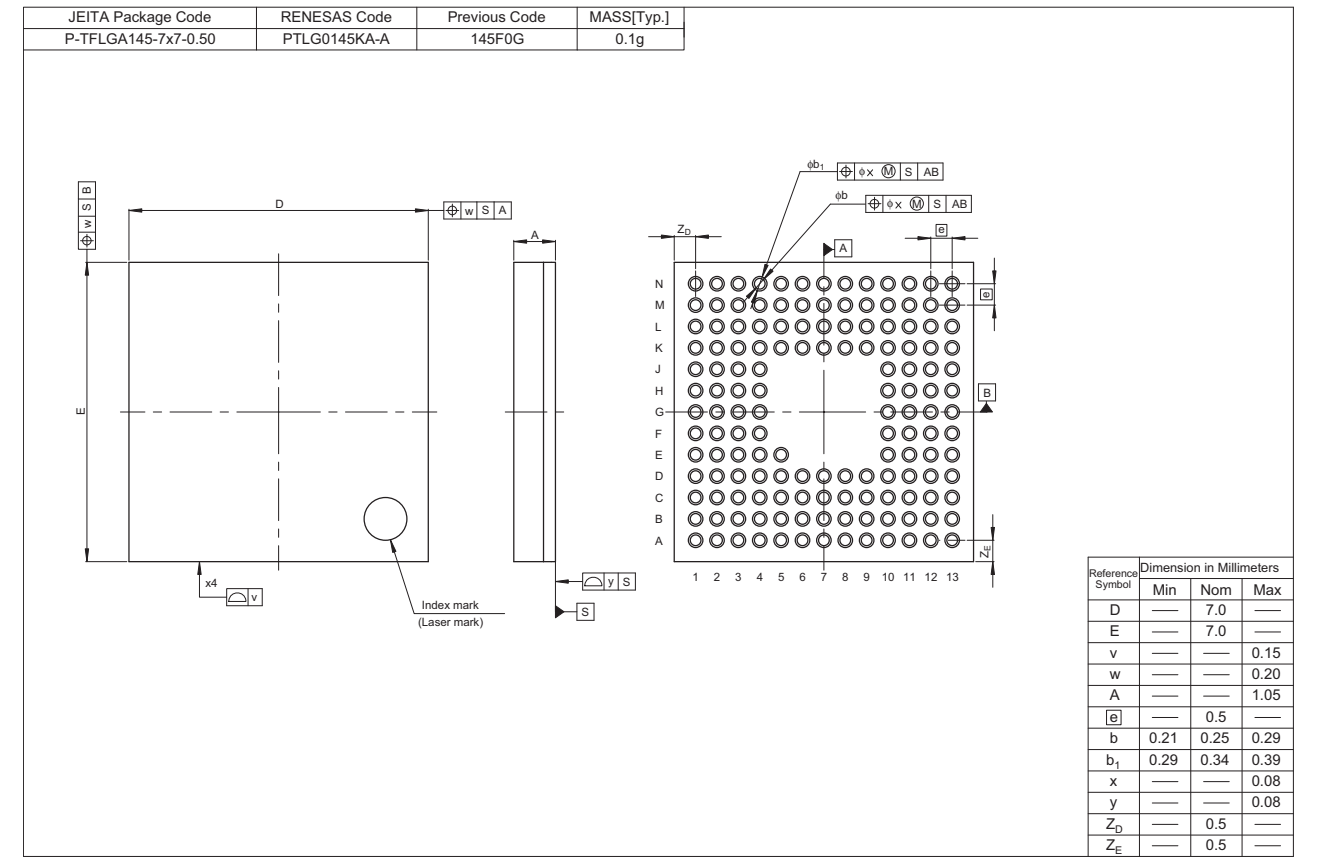
Figure 1.1 LGA 145-pin
