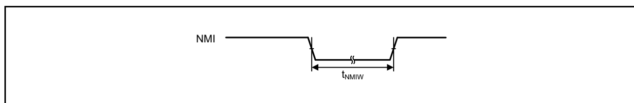
Figure 2.36 NMI interrupt input timing
