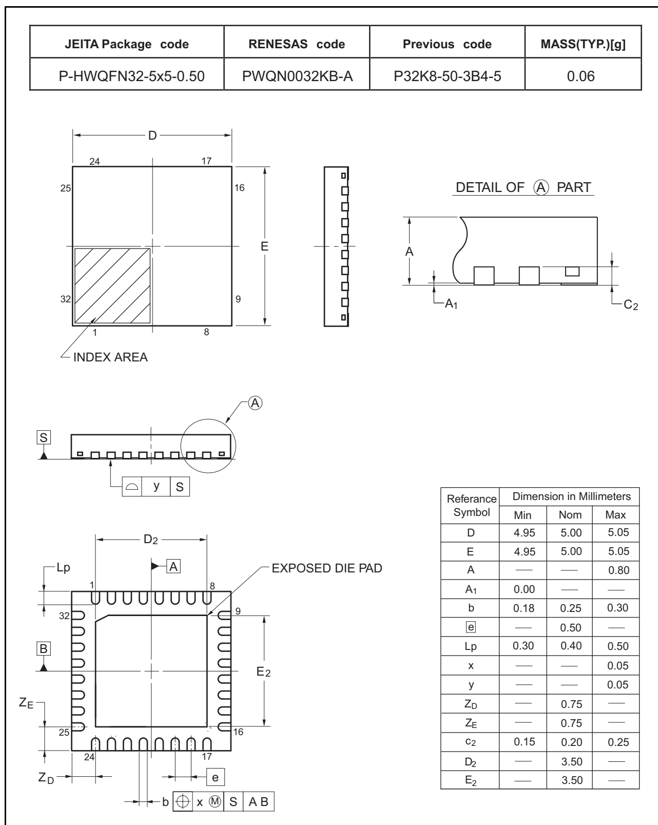
Figure 1.6 QFN 32-pin
