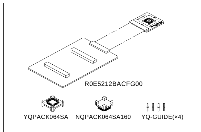
Figure 1 Package components of the R0E5212BACFG00
