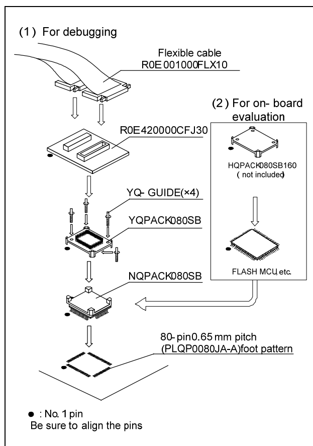
Figure 2 Usage of the R0E420000CFJ30
