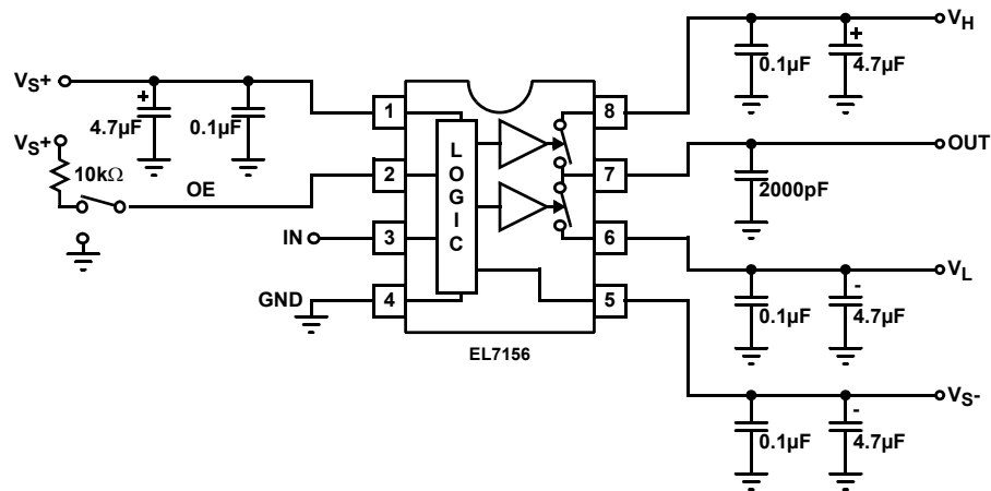
Standard Test Configuration
