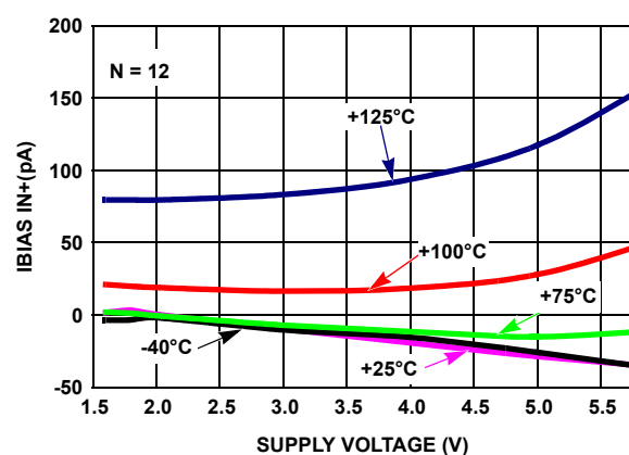
FIGURE 6. I_{B+} vs SUPPLY VOLTAGE vs TEMPERATURE
