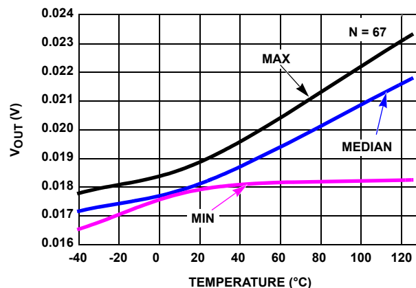
FIGURE 34. V_{OUT} LOW vs TEMPERATURE, R_L = 10k , V_S = +2.5V
