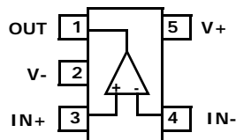
ISL28133 (5 LD SOT-23) TOP VIEW
