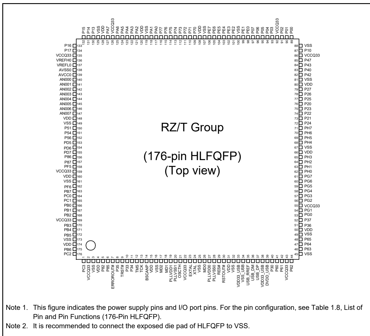
Figure 1.3 Pin Arrangement (176-pin HLFQFP)
