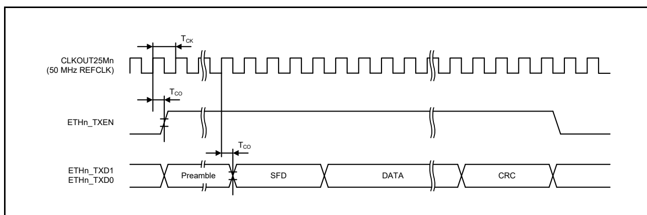
Figure 2.71 RMII Transmission Timing
