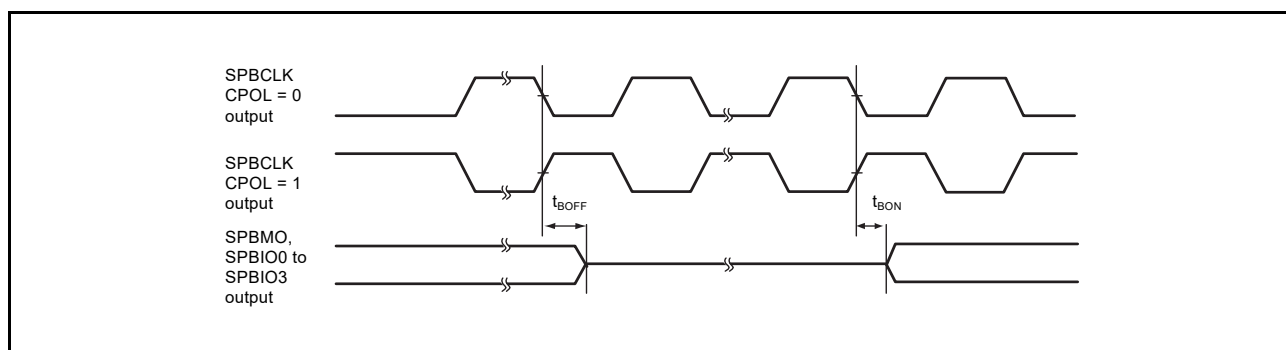
Figure 2.63 SPIBSC Buffer On/Off Timing (CPHAT = 0, CPHAR = 1)
