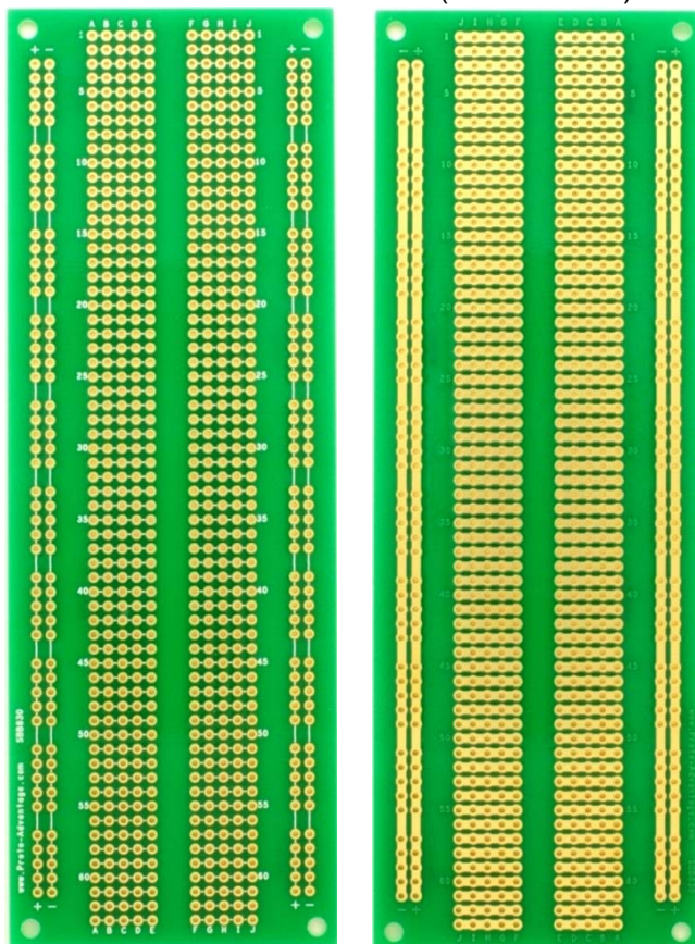
Full size breadboard match (P/N: SBB830)
