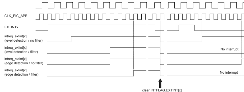
Figure 21-2. Interrupt Detections
