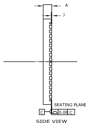
COMMON DIMENSIONS (Unit of Measure = mm)
