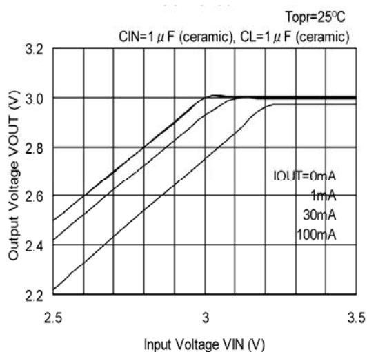
XC6219x302
