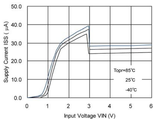
XC6219x302
