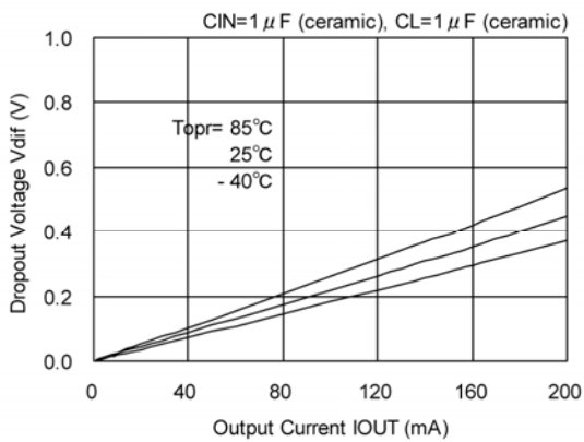
XC6219x302
