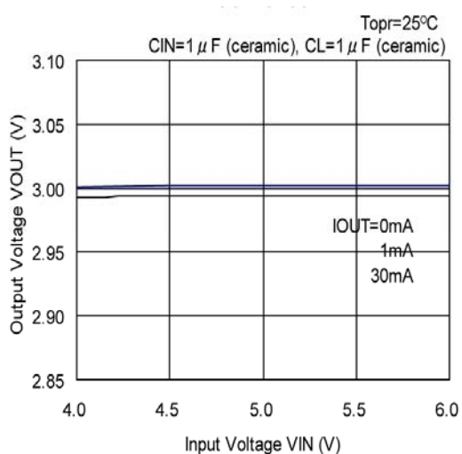
XC6219x302
