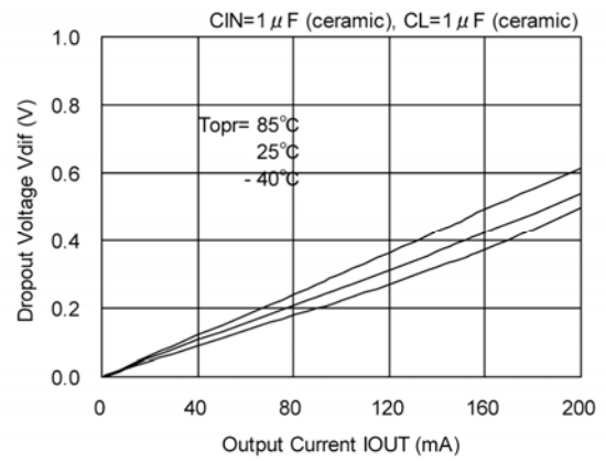
XC6219x252
