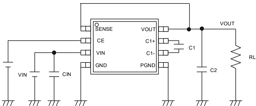
CIRCUIT③
