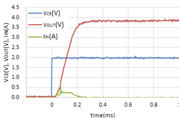
C_{IN}=4.7\mu\text{F} , C_{OUT}=10\mu\text{F} , T_{opt}=25^\circ\text{C} , R_{LOAD}=380\Omega
