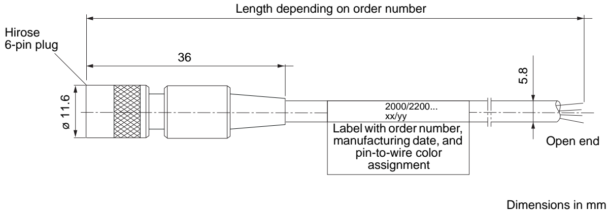
Fig. 1: Cable Overview
