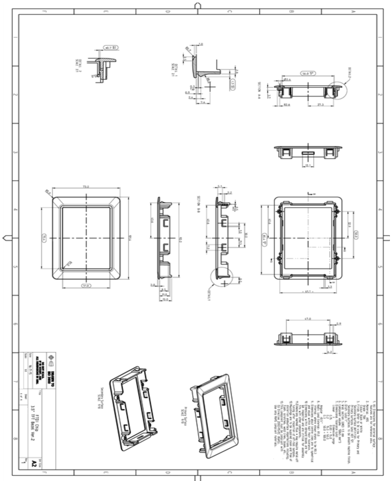
Figure 5-2 – Bezel dimensions
