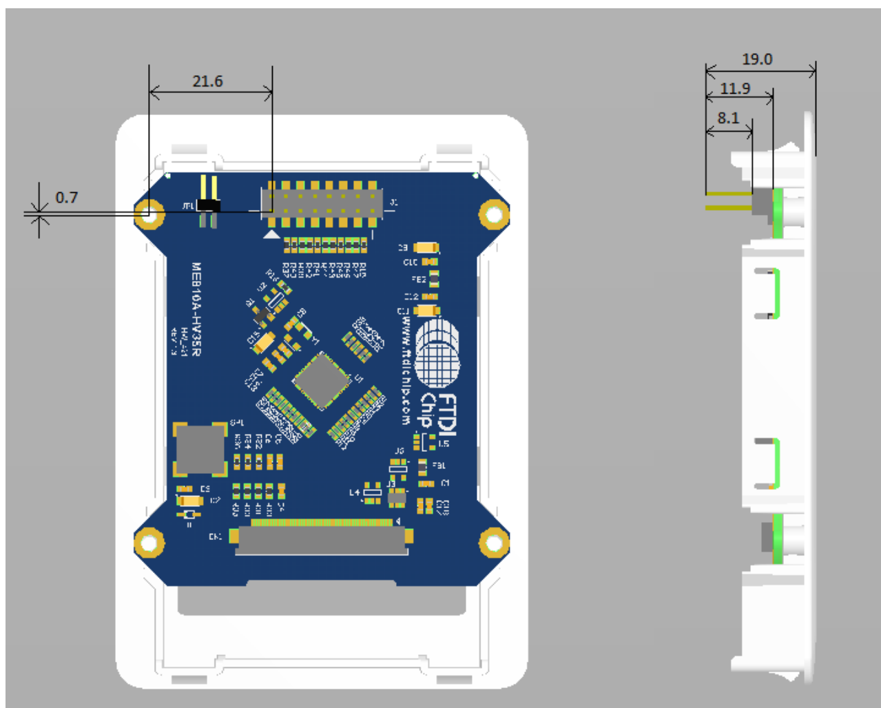
Figure 5-1 – J1 Pin Header Dimensions
