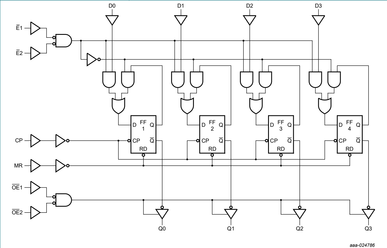
Fig. 4. Logic diagram
