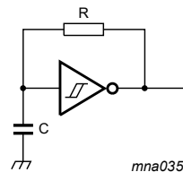
Fig. 12. Relaxation oscillator
