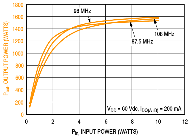
Figure 12. CW Output Power versus Input Power and Frequency
