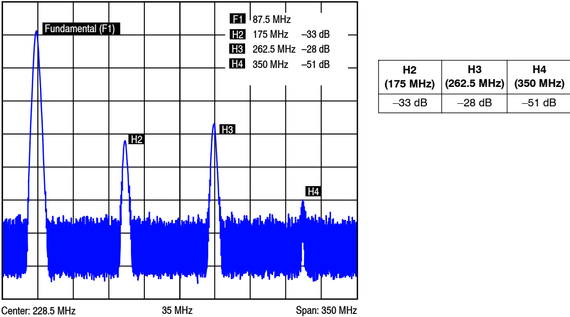
Figure 15. 87.5 MHz Harmonics @ 1300 W CW
