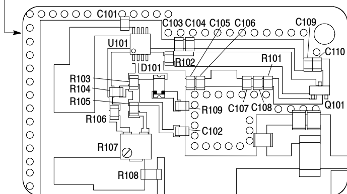
Temperature Compensation Detail
