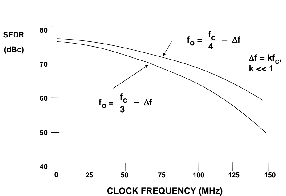
Figure 13: Worst Harmonic vs. Clock Frequency for f_o = f_c/3 - \Delta f and f_o = f_c/4 - \Delta f
