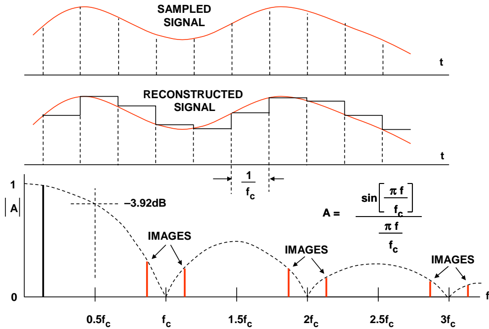
Figure 14: DAC \sin(x)/x Roll Off (Amplitude Normalized)
