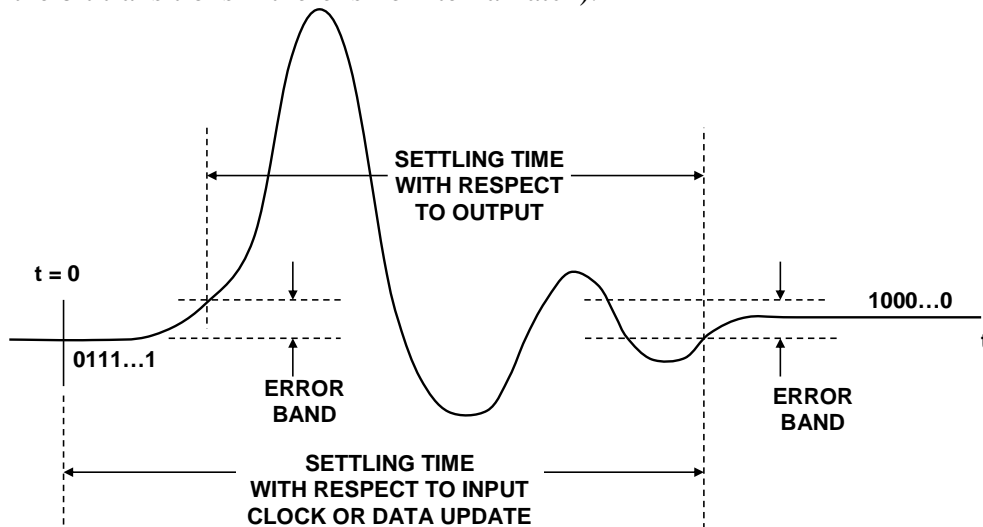
Figure 2: DAC Mid-Scale Settling Time
