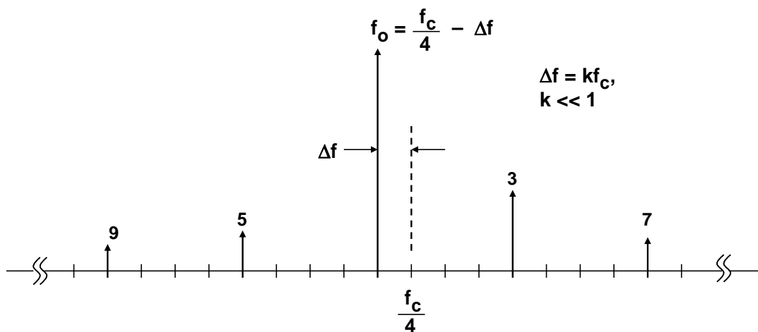
Figure 12: Location of Odd Harmonics for f_o = f_c/4 - \Delta f
