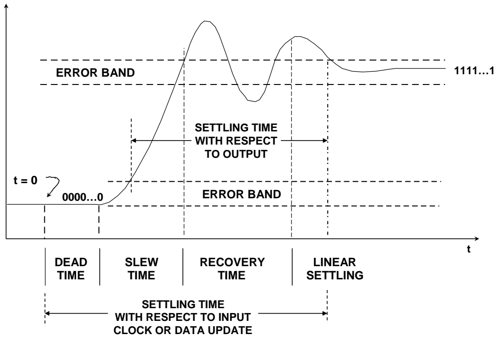
Figure 1: DAC Full-Scale Settling Time
