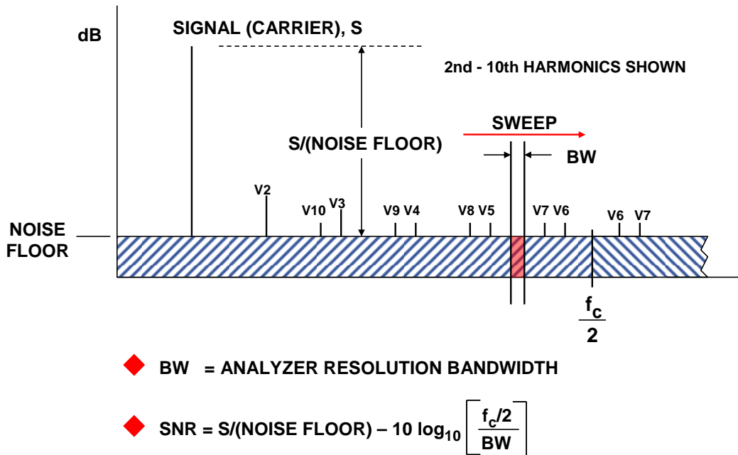
Figure 7: Measuring DAC Distortion and SNR with an Analog Spectrum Analyzer
