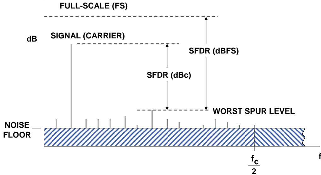
Figure 6: Measuring DAC Spurious Free Dynamic Range (SFDR)
