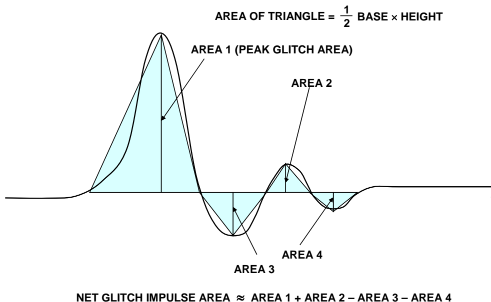
Figure 3: Glitch Impulse Area
