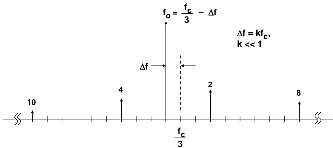
Figure 11: Location of Even Harmonics for f_o = f_c/3 - \Delta f
