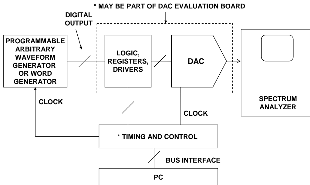
Figure 5: Test Setup for Measuring DAC Distortion and Noise
