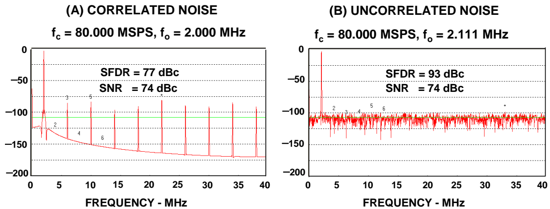
Figure 9: Correlated (A) and Uncorrelated (B) Quantization Noise Spectrum of an Ideal 12-Bit DAC
