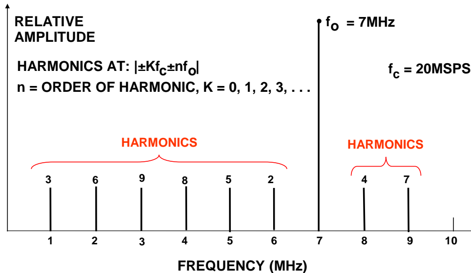
Figure 8: Location of First 9 Harmonic Products: Output Signal = 7 MHz, DAC Update Rate = 20 MSPS
