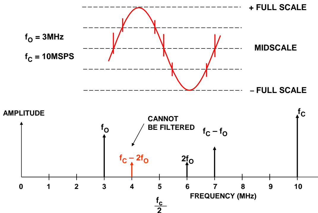
Figure 4: Effect of Code-Dependent Glitches on Spectral Output
