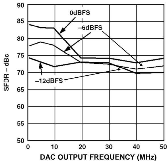
Figure 10: AD9777 16-bit TxDAC™ SFDR, Data Update Rate = 160 MSPS
